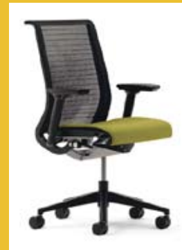
CRITERION
